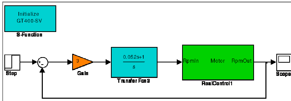
Matlab control interface for the second order system root locus correction
